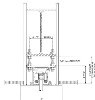
STANDARD DETAIL MANUAL OPERATION
