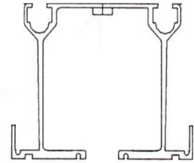
Panelfold Type 7/8 Aluminum Track
